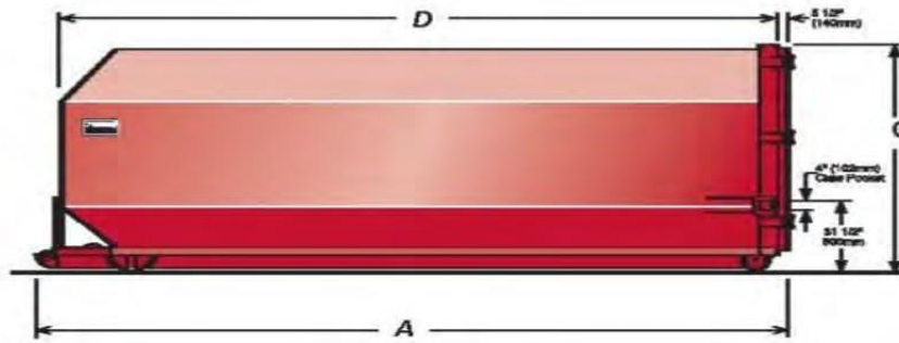
SIDE VIEW
