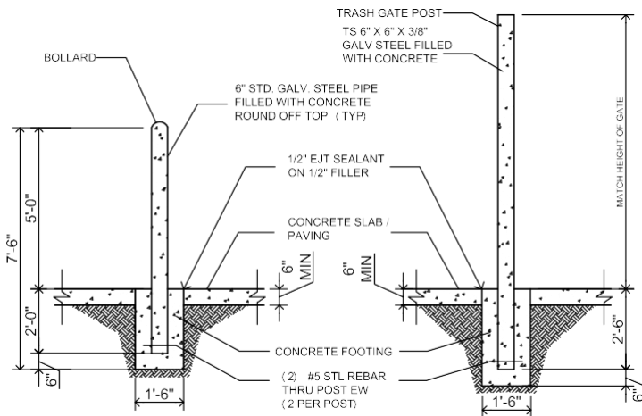
BOLLARD/POST BASE
