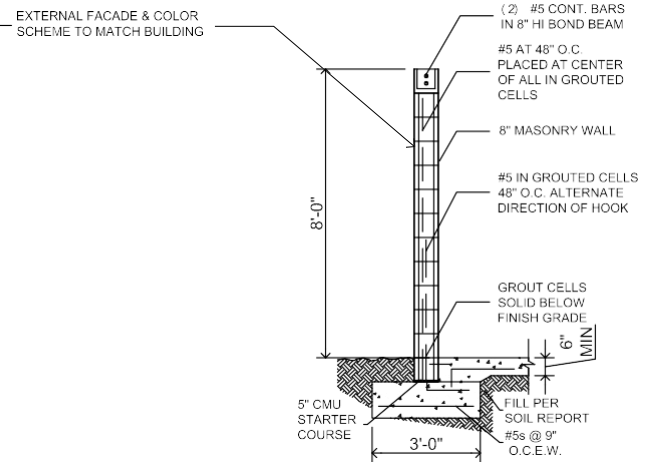
SECTION
