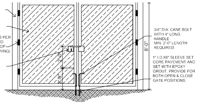
CANE BOLT DETAIL
