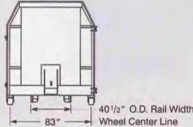
Container End Universal Understructure
